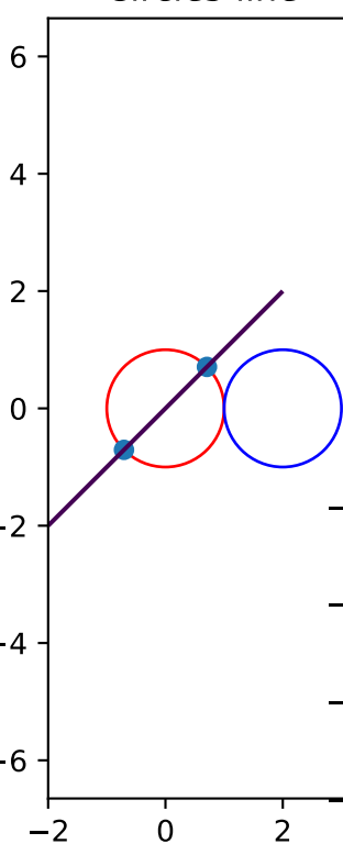
Circles-line
